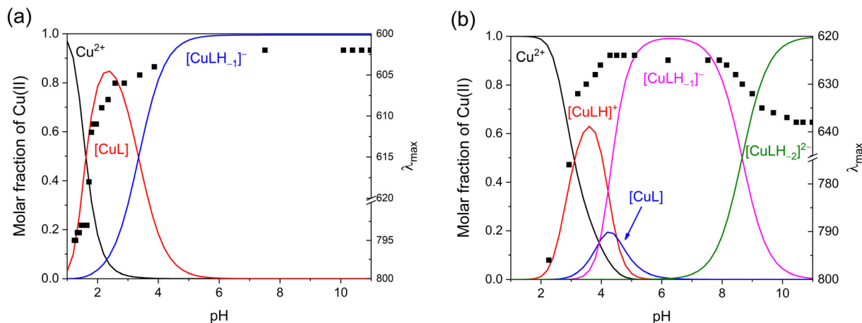
Fig. 1 Distribution of the complexes formed in the Cu(II)–PyHis (a) and Cu(II)–PydiHis (b) systems at a 1:1 metal ion to ligand ratio and the \lambda_{\text{max}} value of the d–d band (■) obtained by UV-vis spectroscopy as a function of pH. c_{\text{Cu(II)}} = 1.81 \text{ mM} , c_{\text{PyHis}} = 1.90 \text{ mM} and c_{\text{PydiHis}} = 1.90 \text{ mM} .
